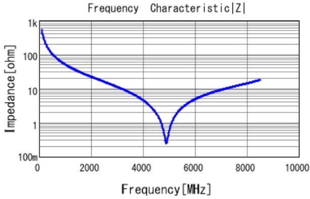
GJM1555C1H3R0BB01 |Z| DCOV, 25degC
