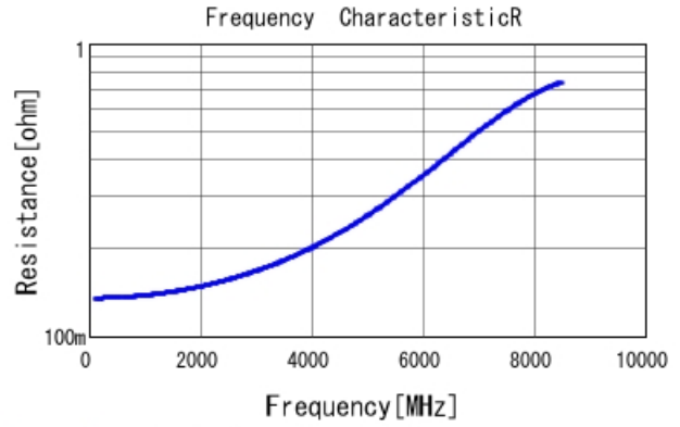
GJM1555C1H3R0BB01 R DCOV, 25degC
