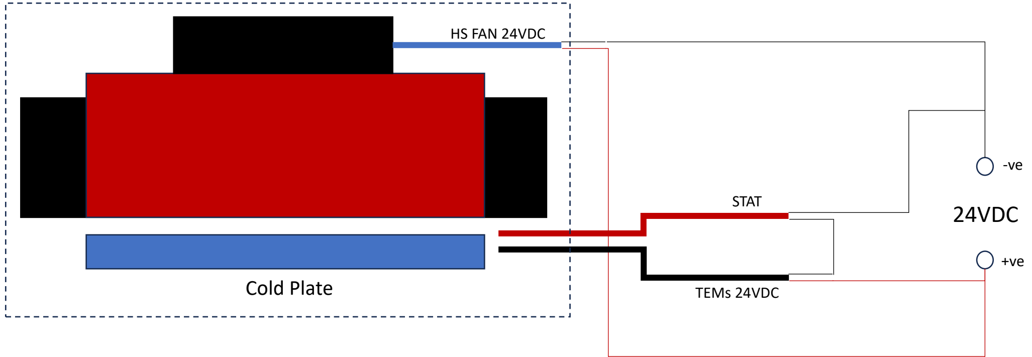
Dt-Ar-075-24 Thermoelectric Assembly
