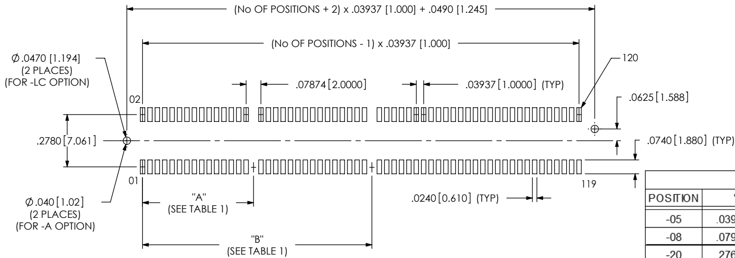
MEC1-160-XX-XX-D-XX SHOWN
