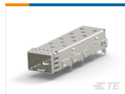
TE Part #2317434-1 SFP+ 1x1 Cage Assy, PCI, Press
