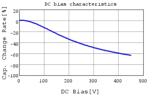
RDED72W104K3K1H03B C-DC bias capchange, 25.0
