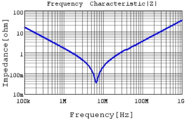
RDED72W104K3K1H03B |Z| DCOV, 25degC
