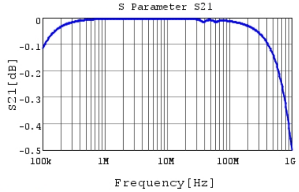
RDED72W104K3K1H03B S21 DCOV, 25degC
