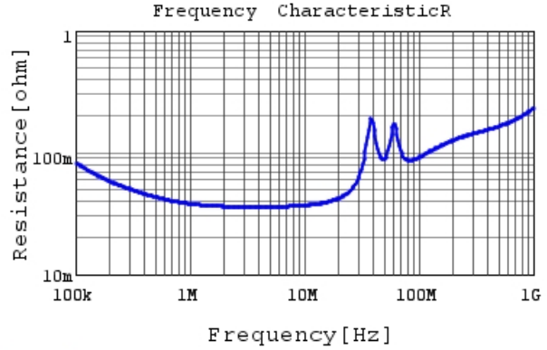
RDED72W104K3K1H03B R DCOV, 25degC
