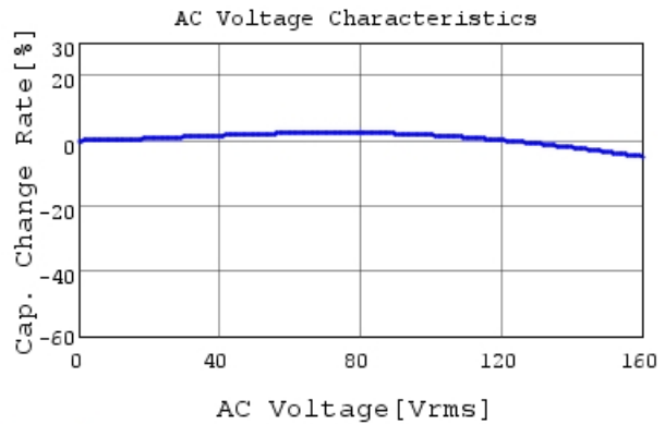
RDED72W104K3K1H03B C-AC Voltage capchange, I
