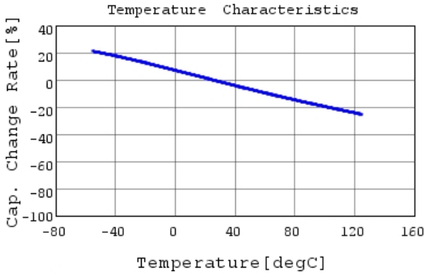
RDED72W104K3K1H03B C-Temp. capchange, DCOV,
