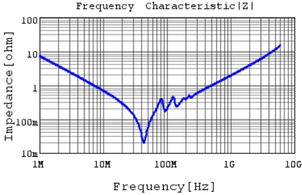
GCM21B5C1H223JA16 |Z| DCOV, 25degC
