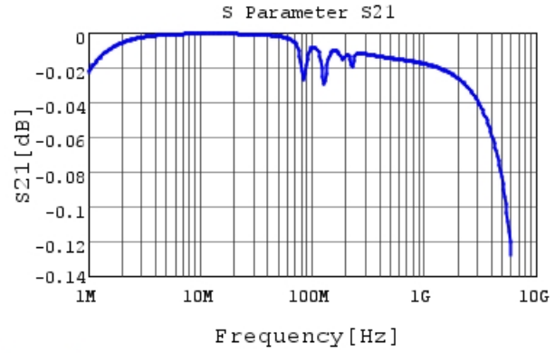
GCM21B5C1H223JA16 S21 DCOV, 25degC
