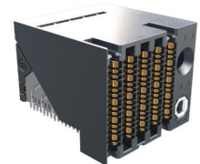
Right Angle Receptacle (Right Guide)
