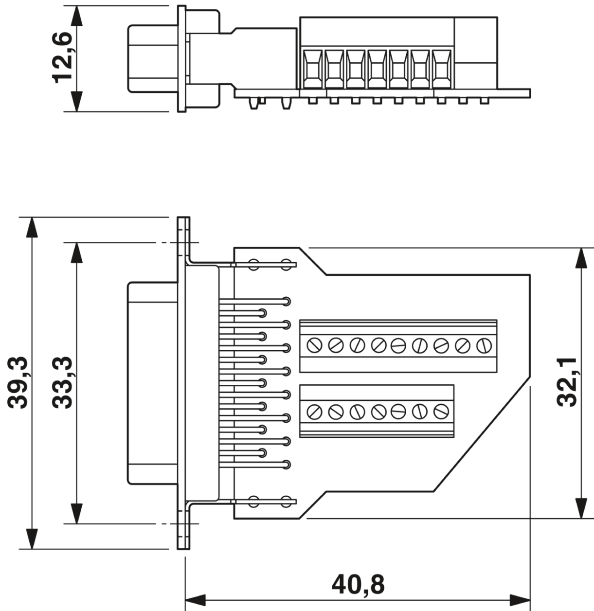
D-SUB contact insert
