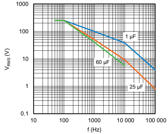
Maximum RMS voltage as function of frequency T_{amb} \leq 85\text{ }^{\circ}\text{C} ; U_r = 250\text{ V}_{AC}
