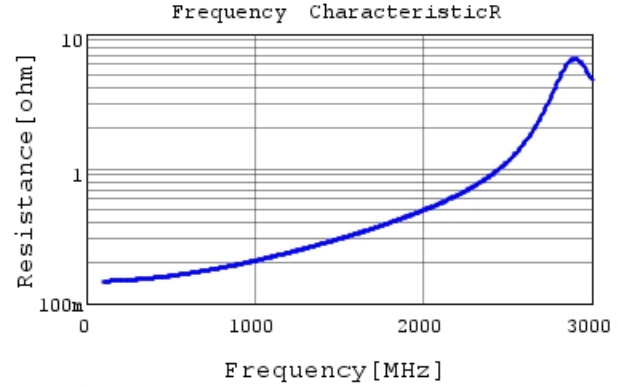
GRM31A5C3A390JW01 R DC0V, 25degC
