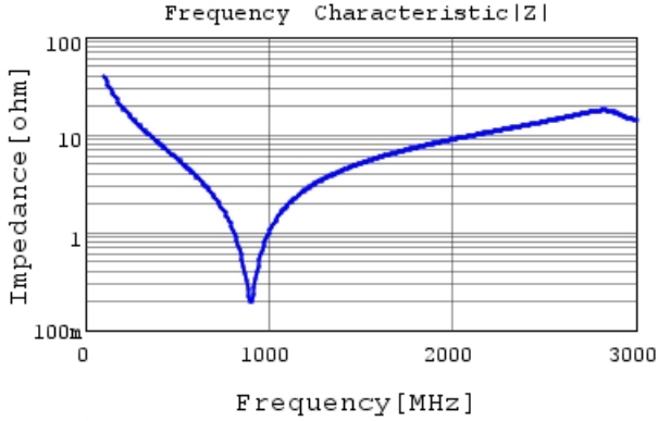
GRM31A5C3A390JW01 |Z| DC0V, 25degC
