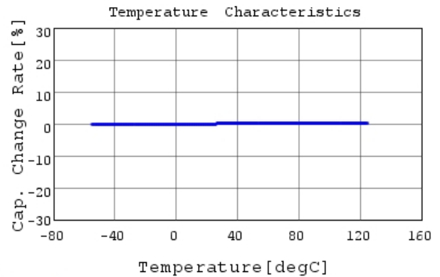
GRM31A5C3A390JW01 C-Temp. capchange, DC0V, 1
