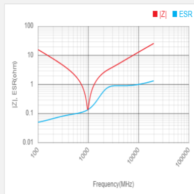
Frequency Characteristics Network Analyzer
