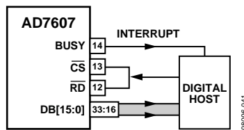
Figure 41. Interface Diagram—One AD7607 Using the Parallel Bus, with \overline{CS} and \overline{RD} Shorted Together
