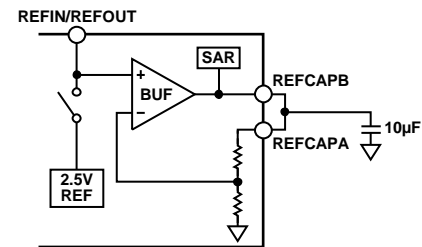
Figure 36. Reference Circuitry
