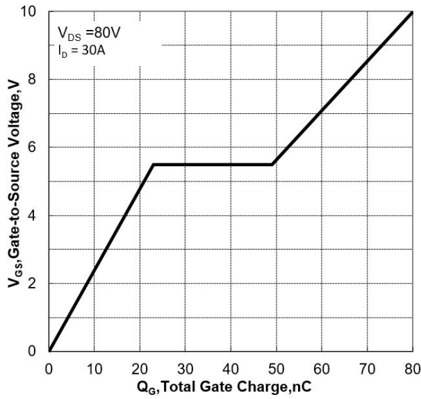
Figure 7 Gate-Charge Characteristics
