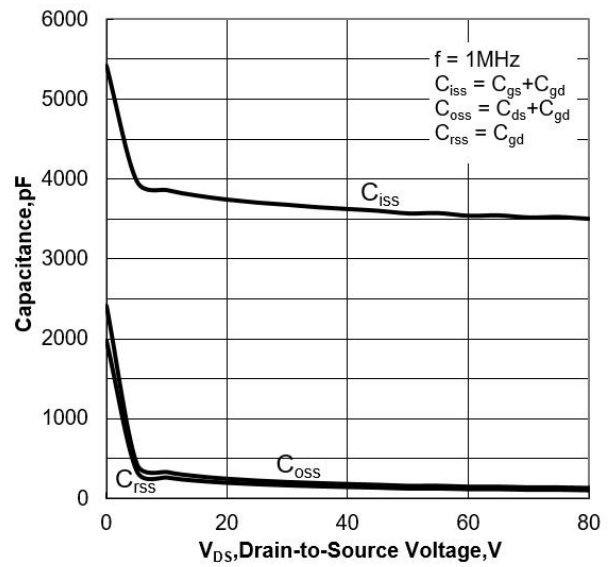
Figure 8 Capacitance Characteristics
