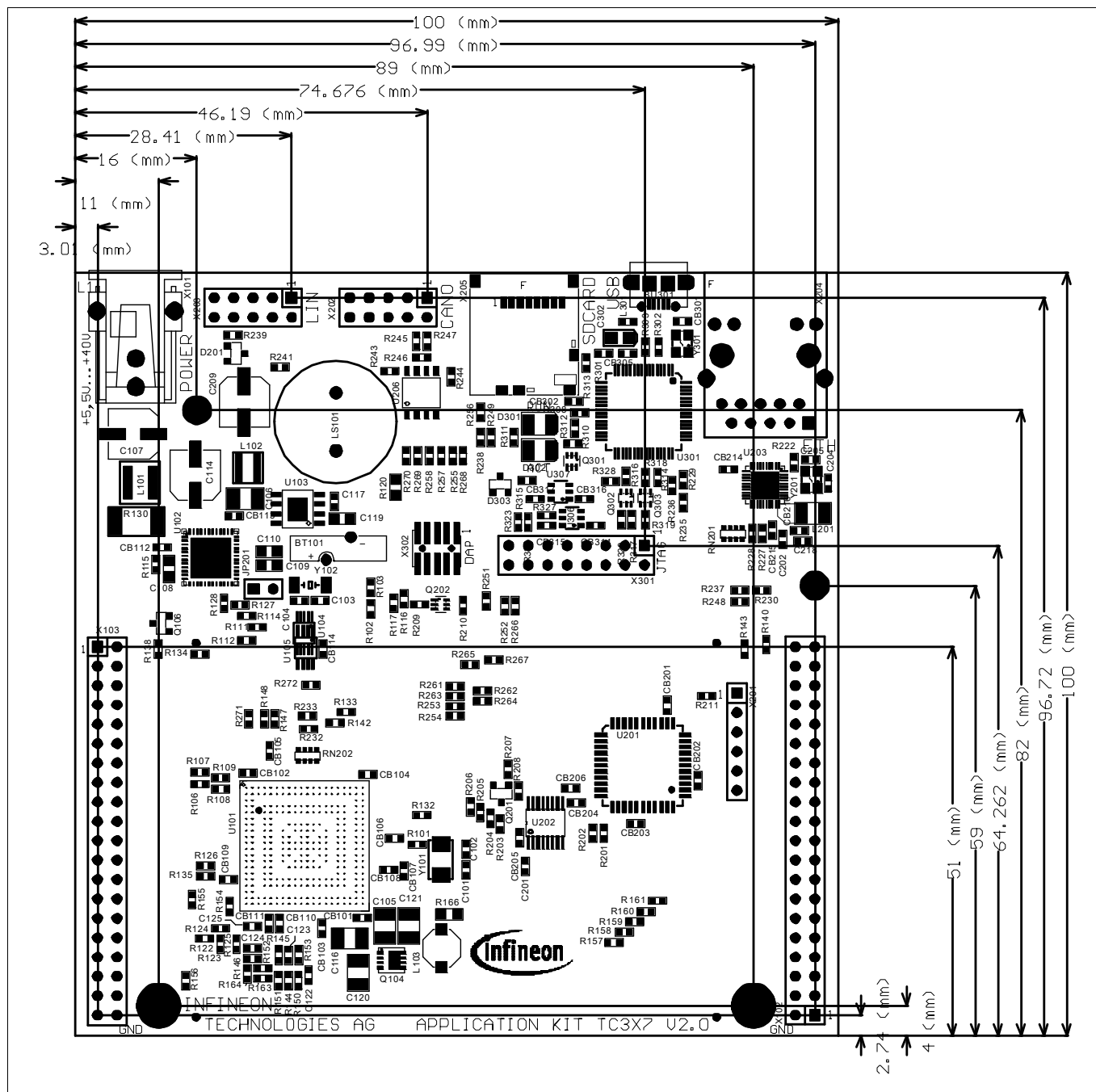
Figure 7-7 Dimensioning (mm)
