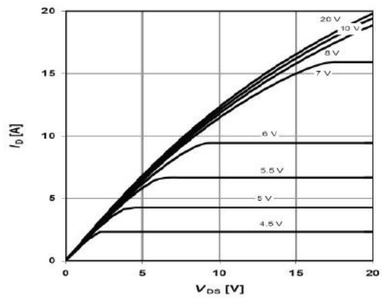
Figure 6. On-Region Characteristics @125°C
