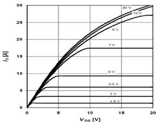
Figure 5. On-Region Characteristics @25°C
