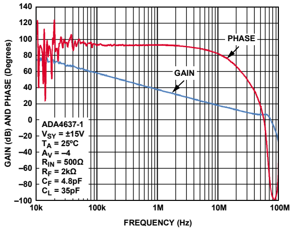
Figure 36. Open-Loop Gain and Phase vs. Frequency
