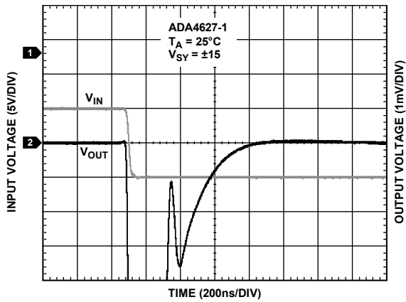
Figure 35. Negative Settling Time to 0.01%
