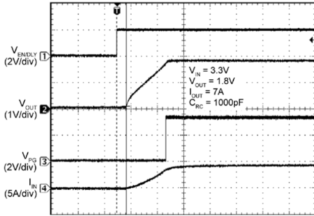
Time (400µs/div)
