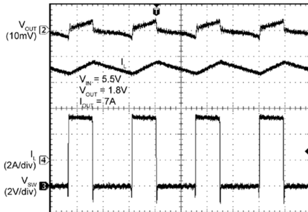
Switching Waveforms
