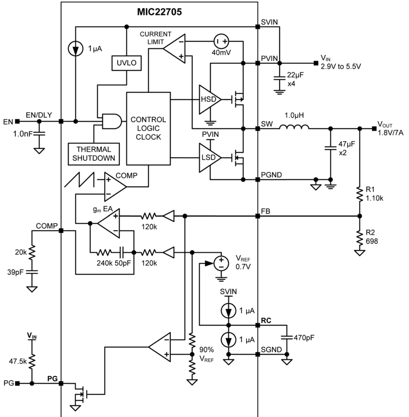
Figure 1. MIC22705 Functional Diagram
