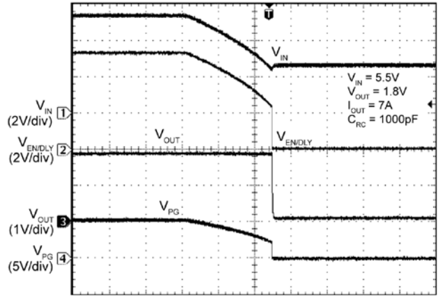
Time (2ms/div)
