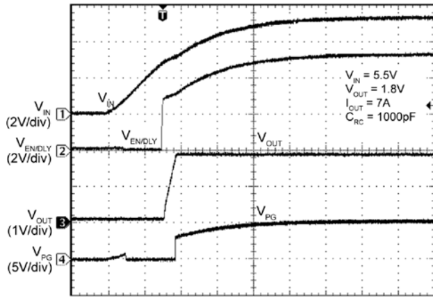
Time (2ms/div)
