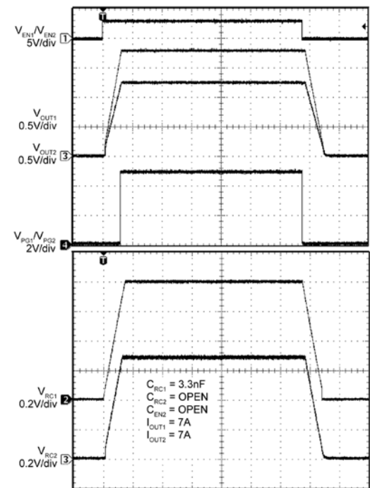
Time (4.0ms/div)
