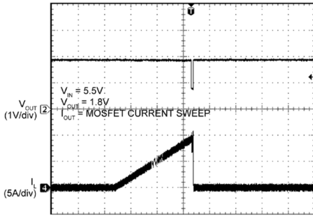
Peak Current-Limit Threshold
