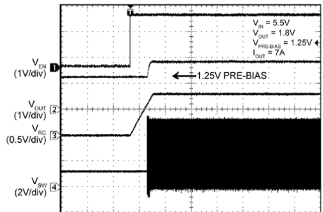
Time (1ms/div)
