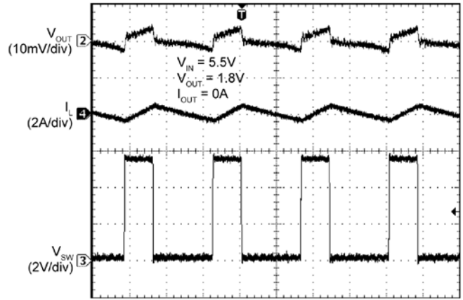
Switching Waveforms
