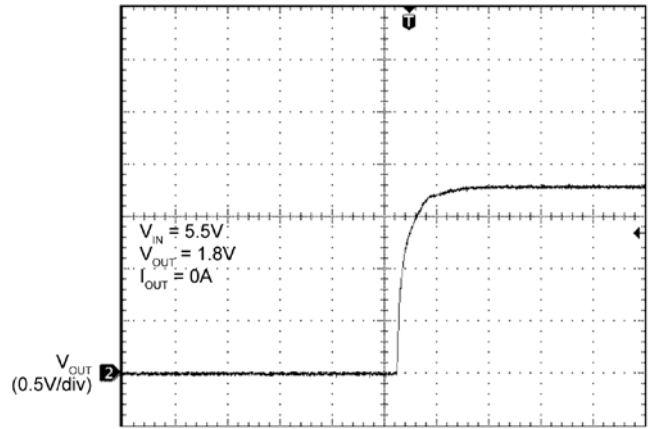
Thermal Shutdown Recovery
