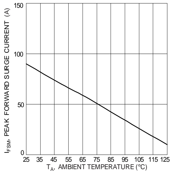
Fig. 6 Non-Repetitive Forward Surge Current Derating Curve
