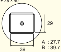
A1263 QFP 28 × 40
