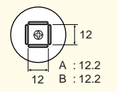
A1262 QFP 12 × 12
