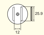
A1261 QFP 20 × 20
