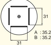
A1260 SOP 8.6 × 18
