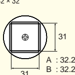
A1265 QFP 32 × 32
