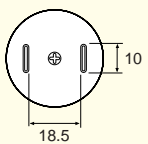
A1257 SOP11 × 21
