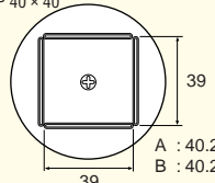
A1264 QFP 40 × 40
