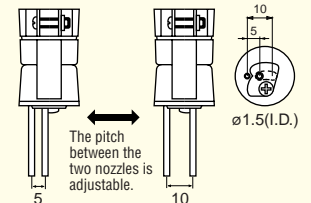
A1325 Dual Single \phi 1.5 \times 5 - 10 Adjustable Pitch
