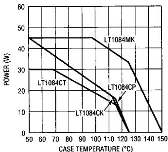
LT1084 Maximum Power Dissipation*
