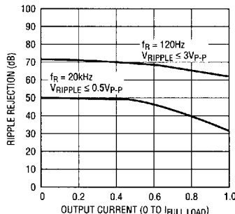
LT1083/4/5-5 Ripple Rejection vs Current
