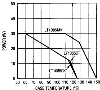
LT1085 Maximum Power Dissipation*
