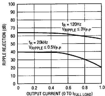
LT1083/4/5-12 Ripple Rejection vs Current
