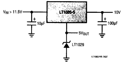
Regulator with Reference
