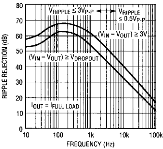
LT1083/4/5-5 Ripple Rejection
