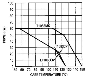
LT1083 Maximum Power Dissipation*
