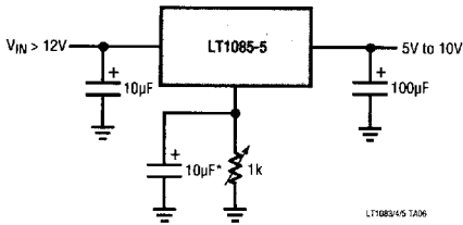
Adjusting Output Voltage
