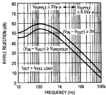
LT1083/4/5-12 Ripple Rejection
