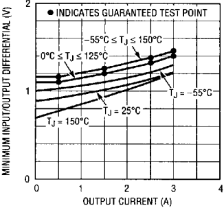
LT1085 Dropout Voltage
