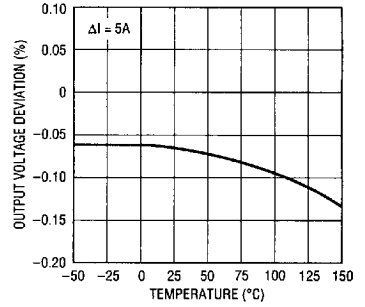
LT1084 Load Regulation
