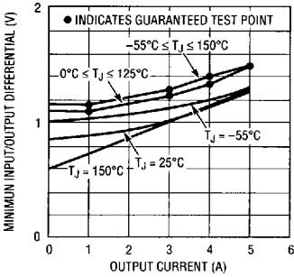
LT1084 Dropout Voltage
