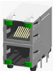
P/N RJSAE-5383-02 SHOWN STACKED 2X1, 8 POSITIONS, WITH SHIELD AND LEDs
