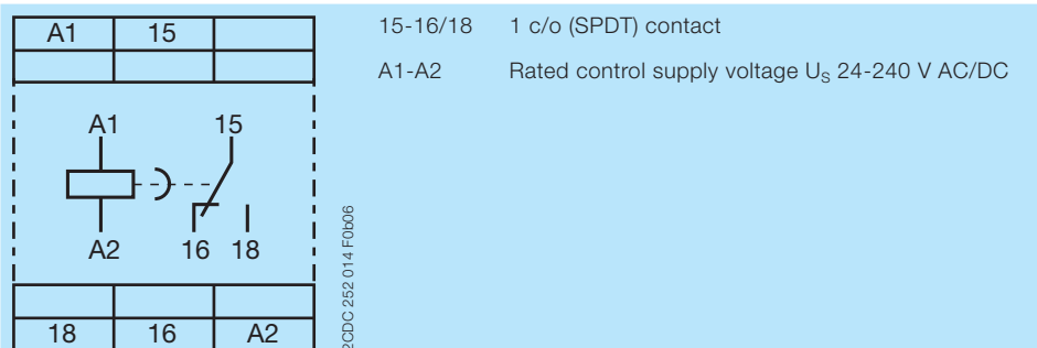
Connection diagram
