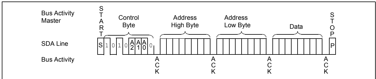
FIGURE 6-1: BYTE WRITE
