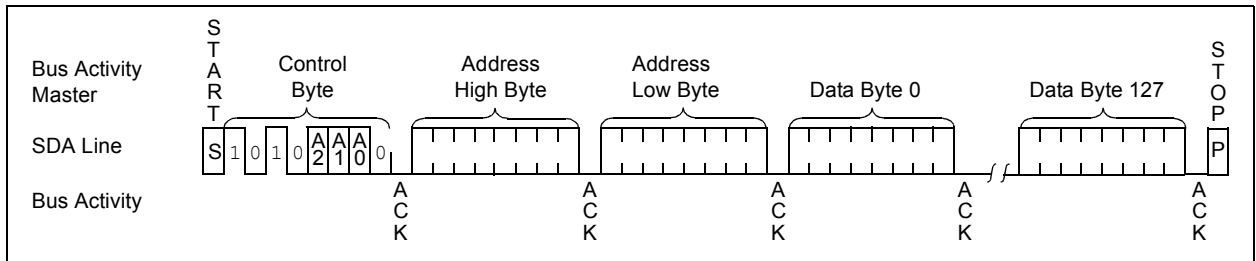
FIGURE 6-2: PAGE WRITE
