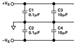
Supply Bypassing
