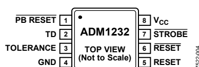
Figure 4. RM-8 Pin Configuration
