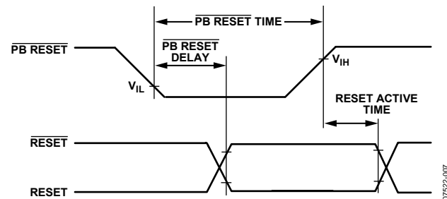
Figure 7. PB RESET
