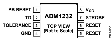
Figure 5. N-8 and R-8 Pin Configuration
