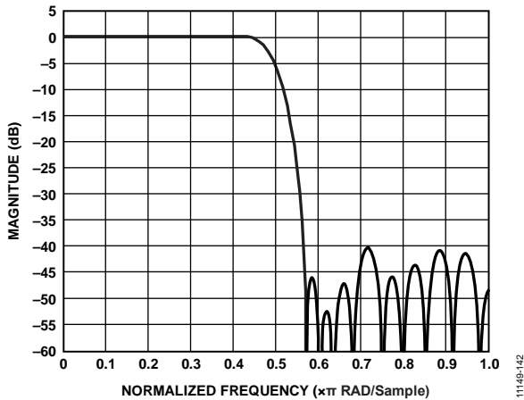
Figure 139. FIR40 2x Interpolation Filter Plot, Complete Frequency Response
