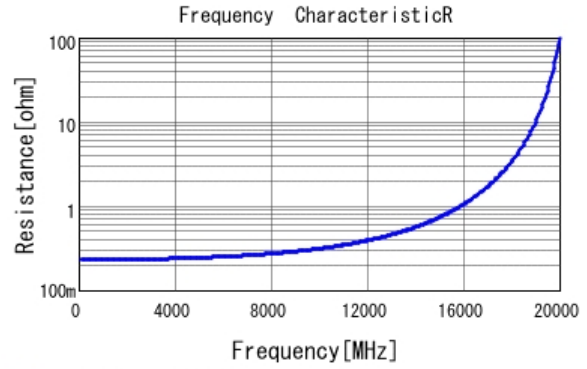
■ GJM1555C1H1R0CB01 R DC0V, 25degC
