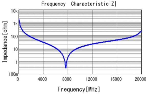
■ GJM1555C1H1R0CB01 |Z| DC0V, 25degC
