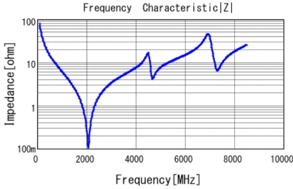
■ GJM1555C1H200GB01 |Z| DC0V, 25degC
