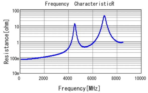
■ GJM1555C1H200GB01 R DC0V, 25degC
