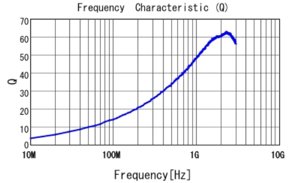
■ LQG18HN6N8J00 Q
