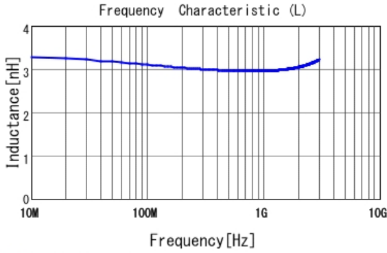
■ LQP03TN3N0B02 L
