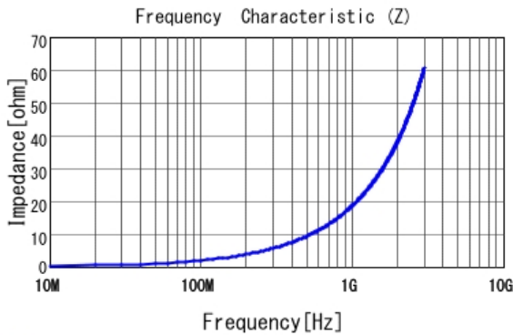
■ LQP03TN3N0B02 |Z|
