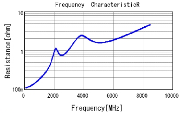
■ GRM2165C2A101JA01 R DCOV, 25degC
