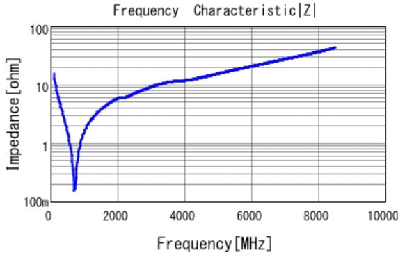
■ GRM2165C2A101JA01 |Z| DCOV, 25degC
