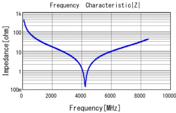
■ GQM1875C2E3R9BB12 |Z| DC0V, 25degC
