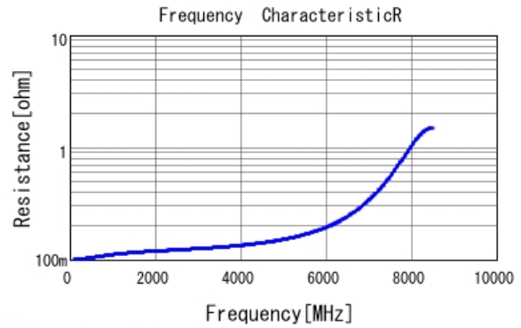
■ GQM1875C2E3R9BB12 R DC0V, 25degC
