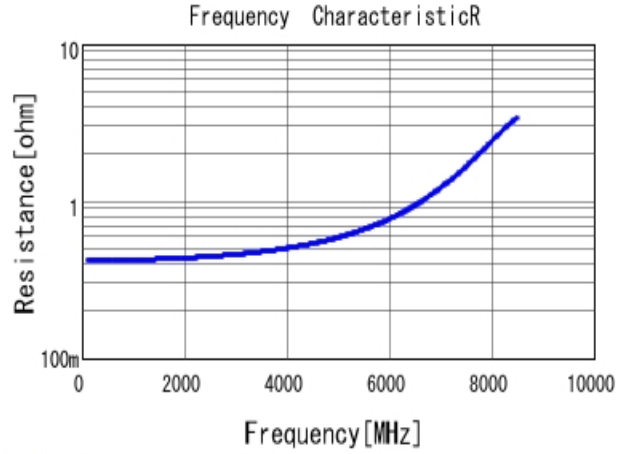
■ GRM1555C1H1R8BA01 R DCOV, 25degC
