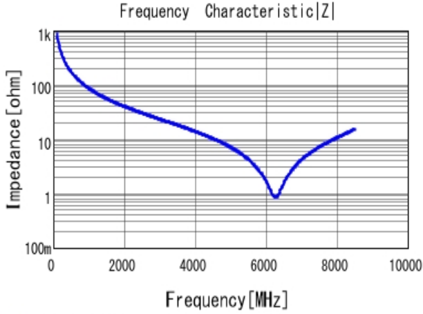
■ GRM1555C1H1R8BA01 |Z| DCOV, 25degC
