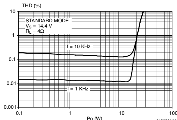
Figure 8. Distortion vs. output power (4 \Omega , STD)
