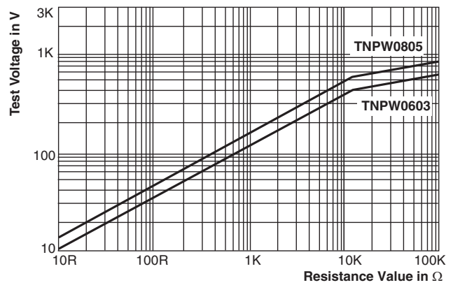
Single-Pulse High Voltage Overload Test 10/700 µs EN 140000 4.27
