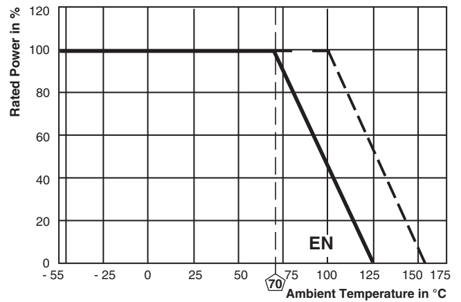
Derating
