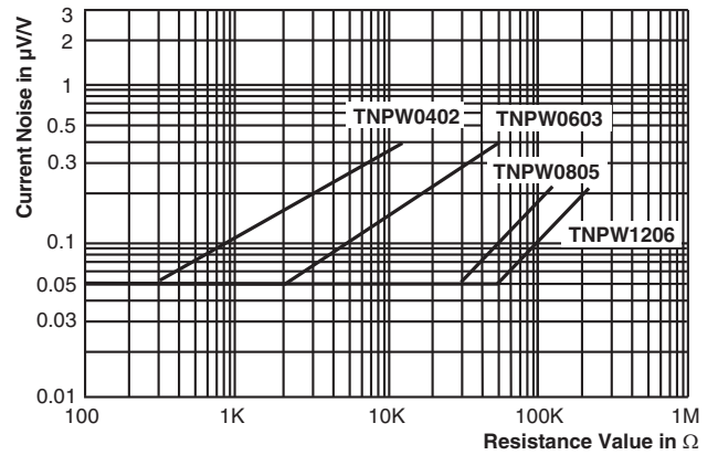
Current Noise
