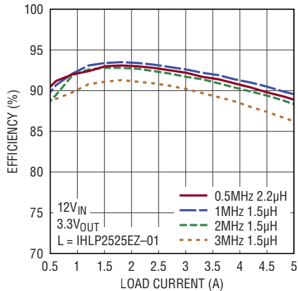
Efficiency at Different f_{sw}
