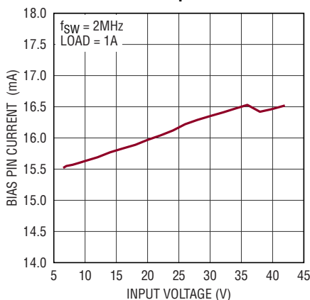
Bias Pin Current per Channel
