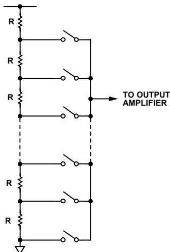
Figure 29. Resistor String
