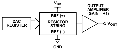
Figure 28. DAC Architecture
