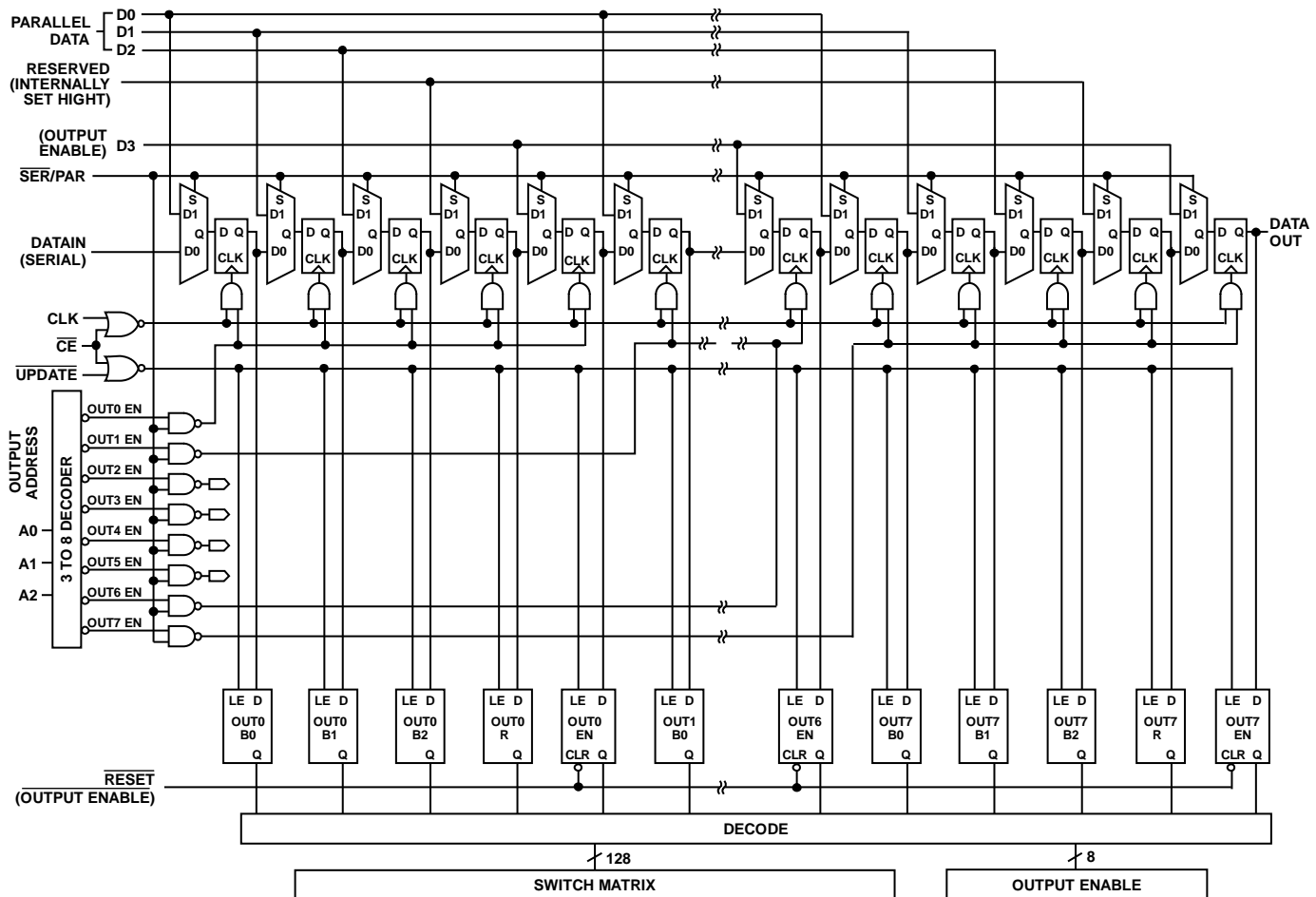
Figure 6. Logic Diagram
