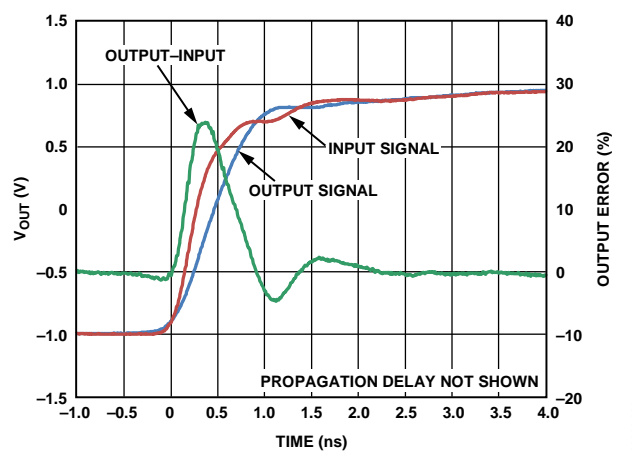
Figure 24. ADV3229 Settling Time
