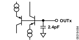
Figure 62. Analog Output Disabled
