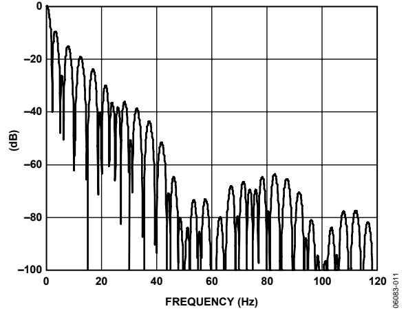
Figure 11. Filter Profile with Update Rate = 4.17 Hz
