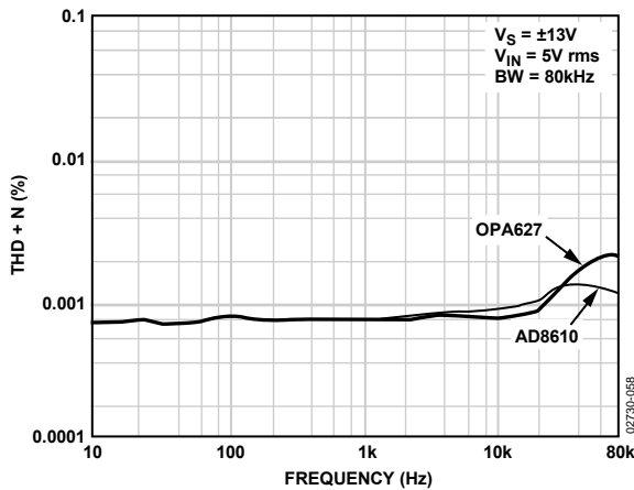
Figure 58. AD8610 vs. OPA627 THD + Noise @ V_{CM} = 0V
