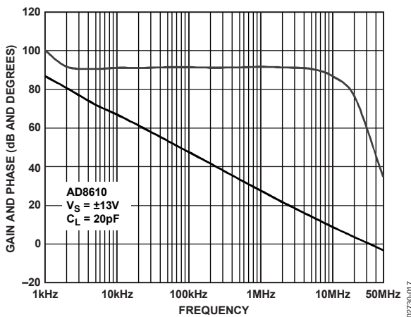
Figure 17. Open-Loop Gain and Phase vs. Frequency
