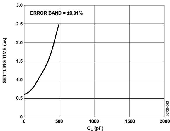
Figure 63. OPA627 Settling Time vs. Load Capacitance
