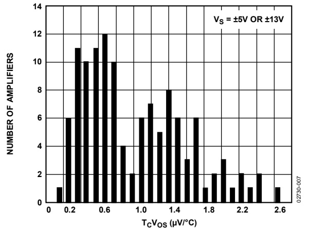
Figure 7. Input Offset Voltage Drift
