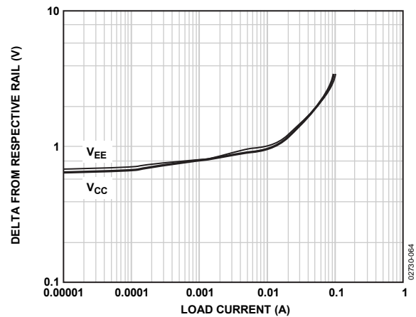
Figure 64. AD8610/AD8620 Dropout from \pm 13 V vs. Load Current
