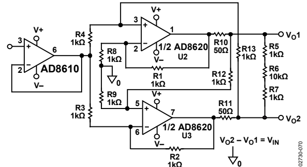
Figure 70. Differential Driver
