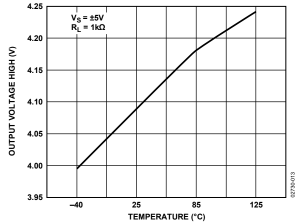
Figure 13. Output Voltage High vs. Temperature
