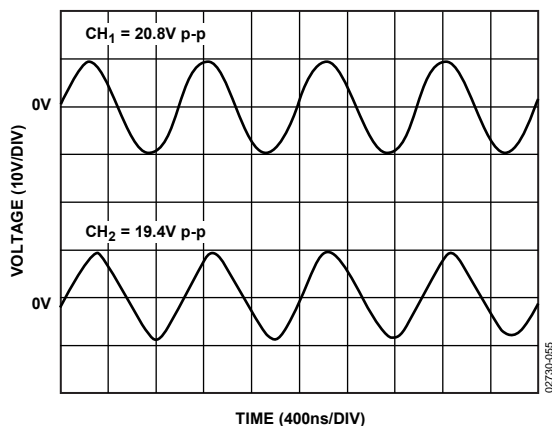
Figure 55. AD8610 FPBW
