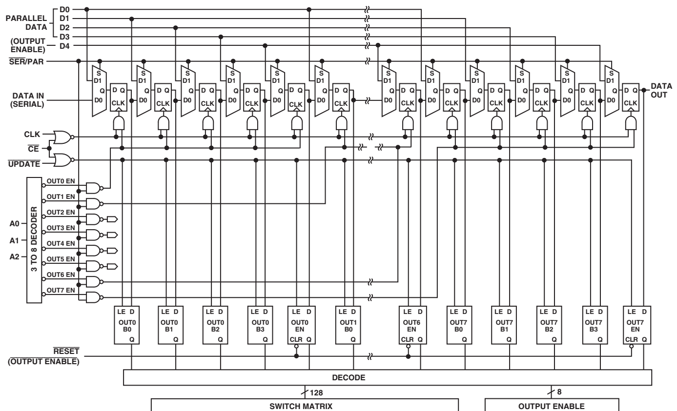
Figure 4. Logic Diagram
