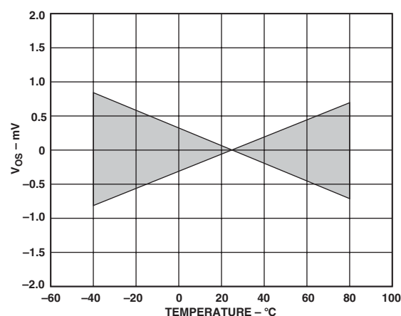
TPC 36. AD8111 Offset Voltage Drift vs. Temperature (Normalized at 25 ^{\circ}C )
