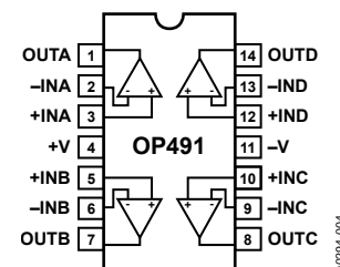
Figure 4. 14-Lead PDIP
