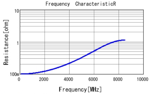
GJM1555C1H5R0BB01 R DCOV, 25degC
