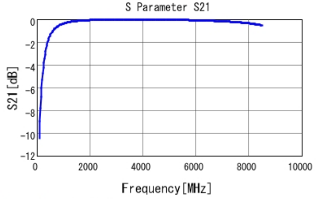
GJM1555C1H5R0BB01 S21 DC0V, 25degC
