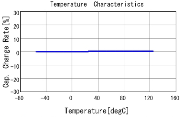
GJM1555C1H5R0BB01 C-Temp. capchange, DC0V, AC1Vrms
