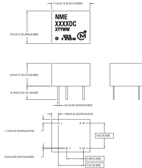
DIP Package
