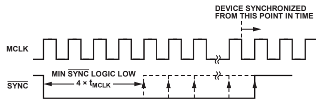
Figure 46. Recommended \overline{\text{SYNC}} Timing
