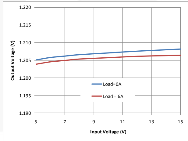
Figure 14. Line Regulation
