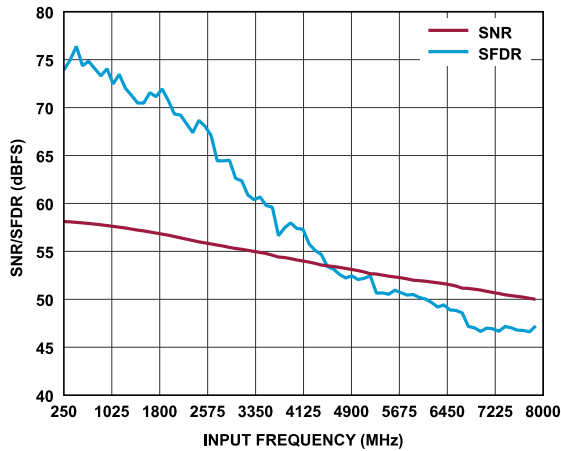
Figure 96. SNR and SFDR vs. Input Frequency with A_{IN} = -1 \text{ dBFS}
