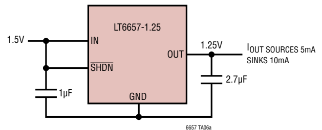
1.5V Minimum Supply Voltage
