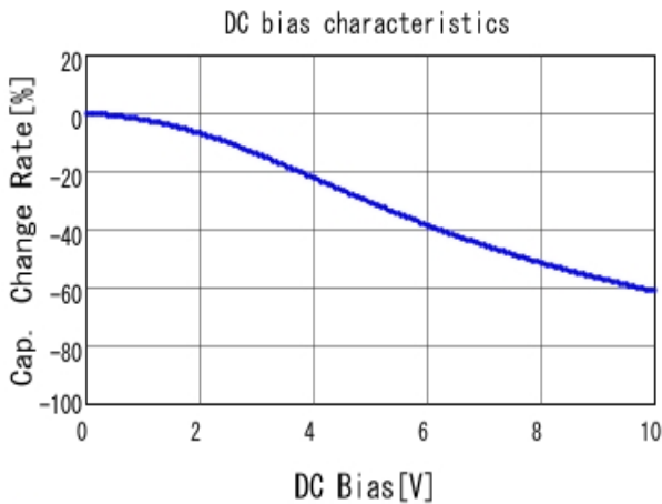
■ GRM316R61A475KE19 C-DC bias capchange, 25.0degC, AC1.
