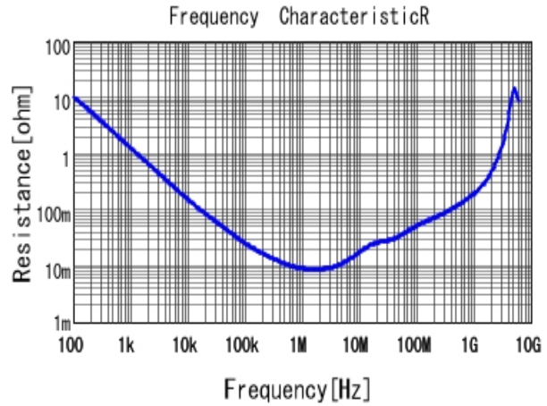
■ GRM316R61A475KE19 R DCOV, 25degC
