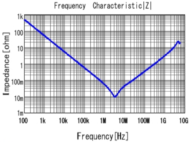
■ GRM316R61A475KE19 |Z| DCOV, 25degC
