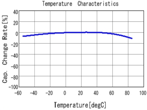
■ GRM316R61A475KE19 C-Temp. capchange, DC0.0V, AC1.0V rm
