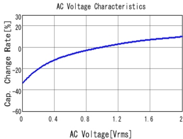
■ GRM316R61A475KE19 C-AC Voltage capchange, DCOV, 25.0d
