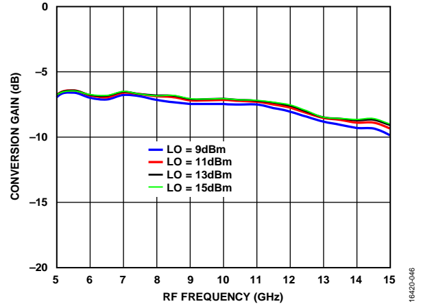
Figure 44. Conversion Gain vs. RF Frequency at Various LO Power Levels, T_A = 25^\circ\text{C}
