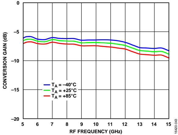
Figure 41. Conversion Gain vs. RF Frequency at Various Temperatures, LO = 13 dBm
